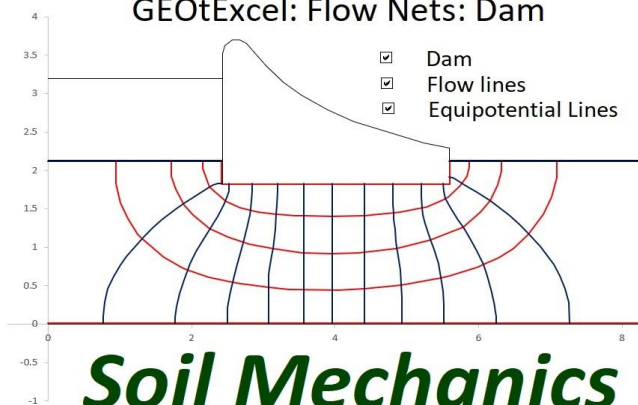
GEOtExcel: Flow Nets: Dam
