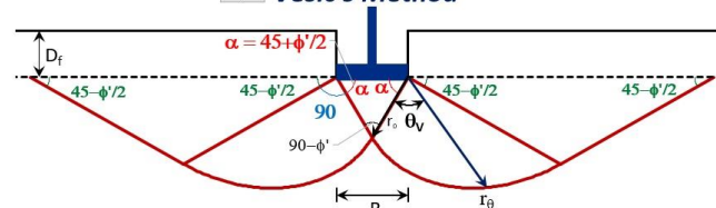
Vesic's Method
